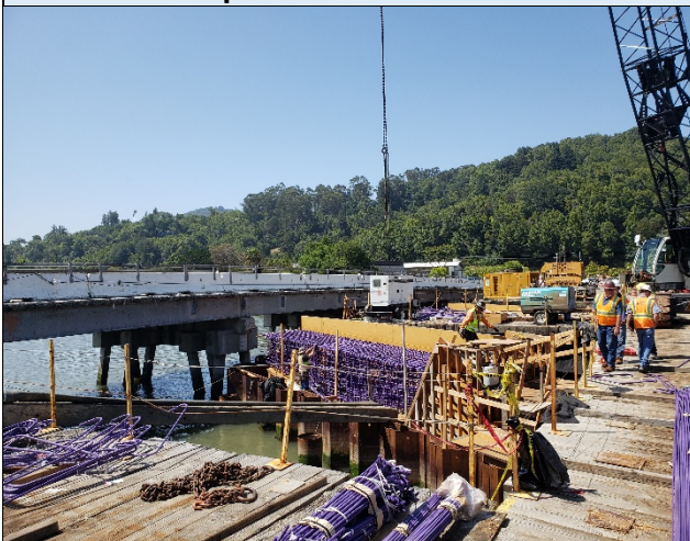
Pier 2 Bent Cap Installation
